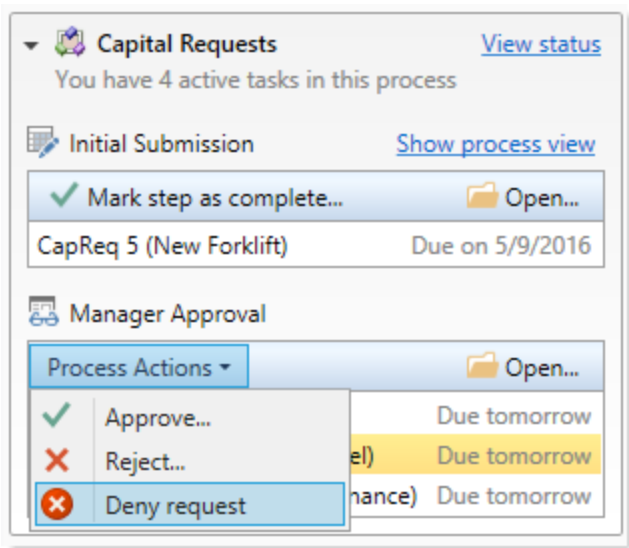
Desktop Client Process task pane
